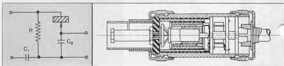
Figure 2. Schematic (left) and cross section (right) of the probe.
